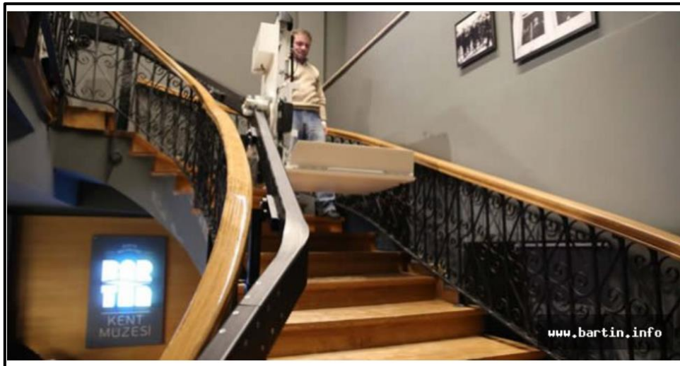
Inclined Curved Platform Lift (Wheelchair) 1 Flat – 2 Stops Indoor
