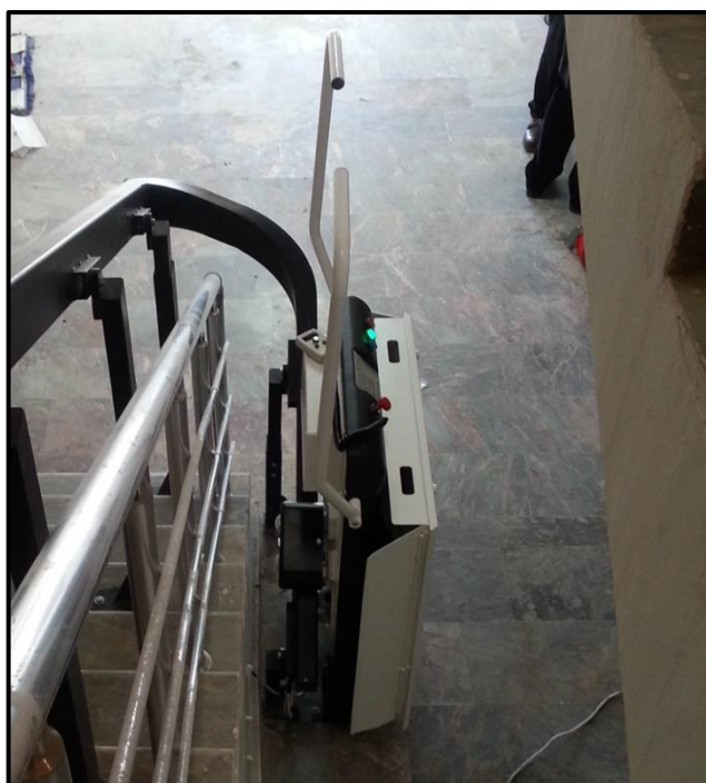
Inclined Curved Platform Lift (Wheelchair) 2 Flats – 3 Stops Indoor
